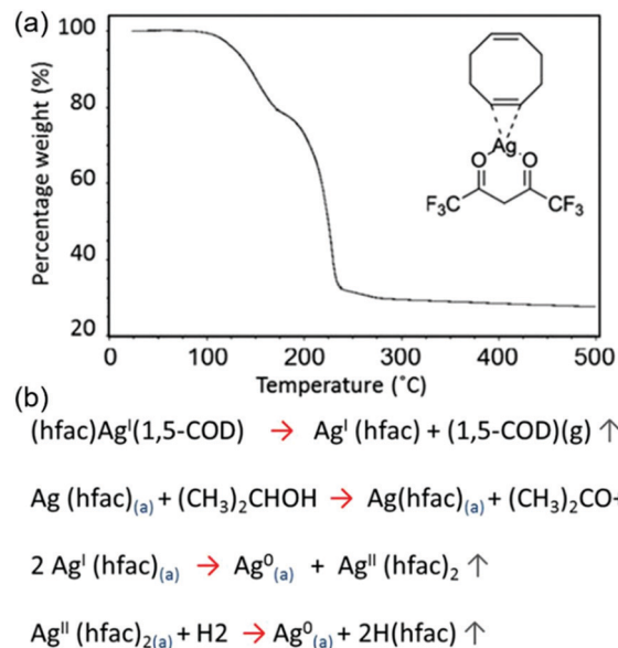
Fig. 19 (a) Thermogravimetric analysis of the pure [(hfac)(1,5-COD)Ag] ink component. (b) The decomposition processes of [(hfac)(1,5-COD)Ag]. Reproduced with permission from ref. 83. Copyright 2016, Rights Managed by Nature Publishing Group.
