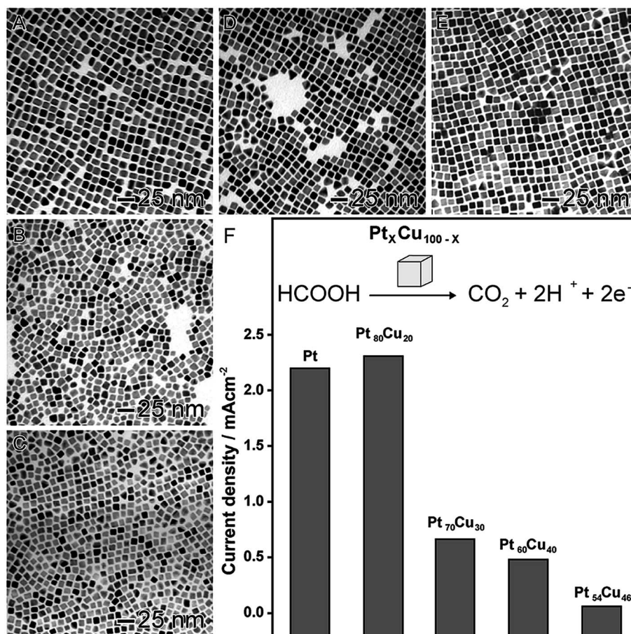
Fig. 3 Effect of NPs composition over catalytic activity. TEM images of bimetallic Pt_xCu_{100-x} nanocubes with controlled compositions: Pt_{100} (A), Pt_{80}Cu_{20} (B), Pt_{70}Cu_{30} (C), Pt_{60}Cu_{40} (D), and Pt_{54}Cu_{46} (E). (F) Maximum current densities for formic acid oxidation employing Pt_xCu_{100-x} nanocubes as electrocatalysts. Adapted from ref. 82 with permission.
