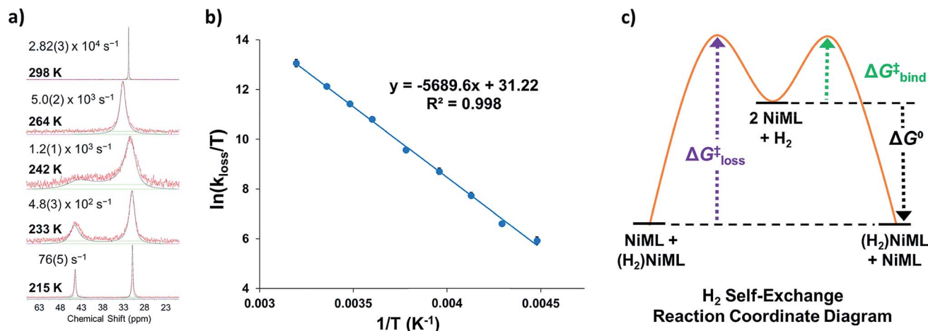
Fig. 3 (a) Selected VT 31 P NMR spectra of 1 under 1 atm H 2 from 215 to 298 K (red lines, toluene- d 8 , 162 MHz) and corresponding simulated spectra (black lines), which were utilized to extract exchange rates at each T (standard deviations in parentheses). (b) Eyring plot of \ln(k_{\text{loss}}/T) vs. 1/T , where k_{\text{loss}} is the first-order rate constant for H 2 loss from 1-H 2 . (c) Proposed reaction coordinate diagram for chemical exchange between (η 2 -H 2 )NiML and NiML via unimolecular H 2 loss.
