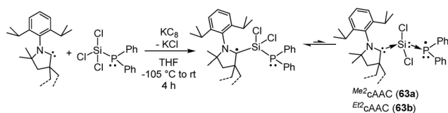
Fig. 17 Radicals of silicon and phosphorus stabilized by cAAC.
