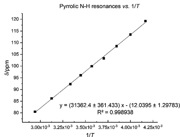
Fig. 7 Temperature dependence of pyrrole ^1\text{H} NMR spectroscopic resonance in 8 between 240 K and 340 K.
