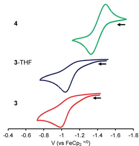
Fig. 3 CVs of 3 , 3-THF and 4 with 0.1 M [ ^{17}\text{Pr}_4\text{N} ][ \text{BAR}_4^{\text{F}} ] electrolyte in DFB (scan rate of 100 mV \text{s}^{-1} ; collected under Ar).
