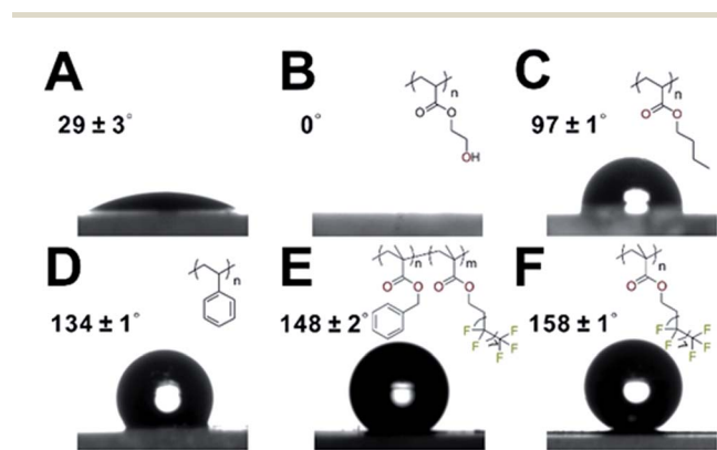
Fig. 5 Water contact angle measurement for UiO-66 (A), UiO-66@PHEA (B), UiO-66@xPBA (C), UiO-66@xPS (D), UiO-66@xP(BzMA- co -PFMA) (E), and UiO-66@xPPFMA (F).
