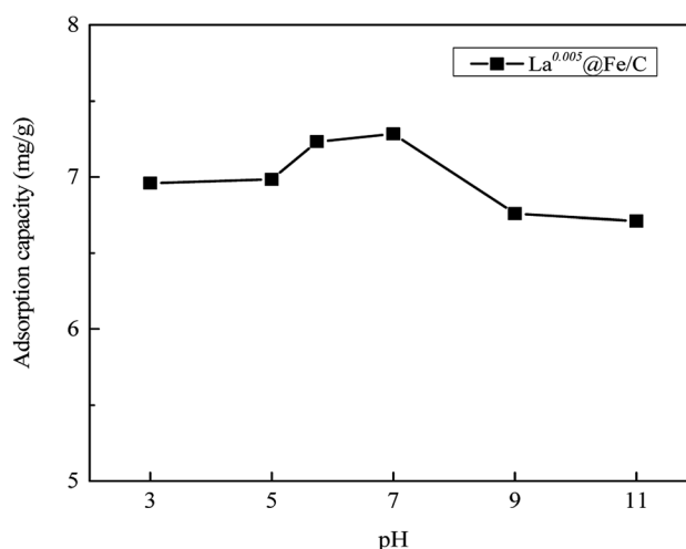
Fig. 7 Influences of pH on phosphate adsorption by \text{La}^{0.005}\text{@Fe/C} .
