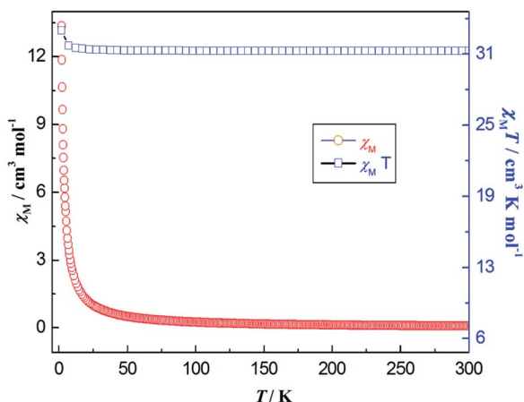
Fig. 14 Thermal variation (temperature dependence) of \chi_M T (□) and \chi_M (○) versus T for coordination polymer 7 under the DC magnetic field of 1000 Oe.
