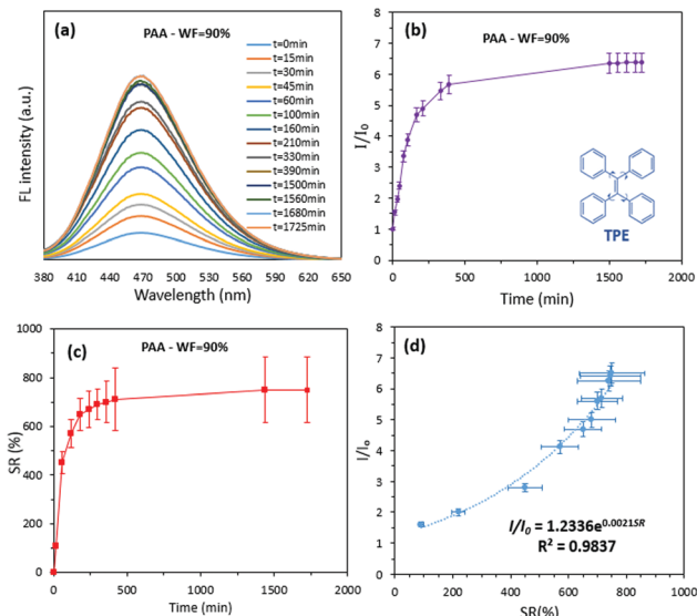
Fig. 2 Change in (a) fluorescent spectra, (b) relative intensity and (c) SR, and (d) the established relationship between the relative fluorescence intensity and the SR for a PAA (film) hydrogel during the swelling process in water–TPE/THF swelling media with water fraction = 90%.
