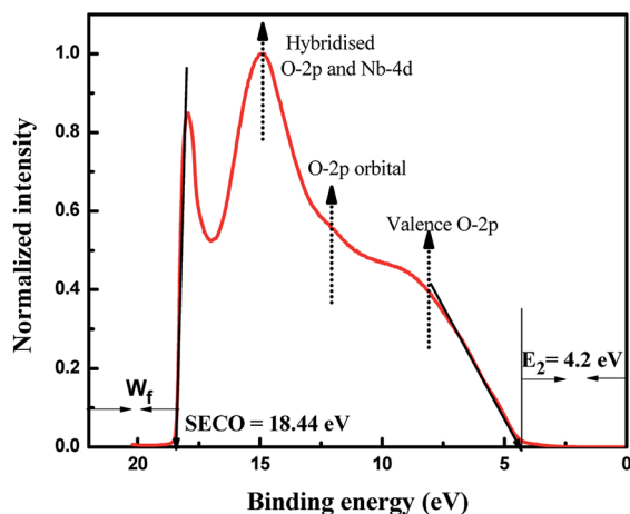
Fig. 4 UPS spectra of \text{Nb}_2\text{O}_5 .
