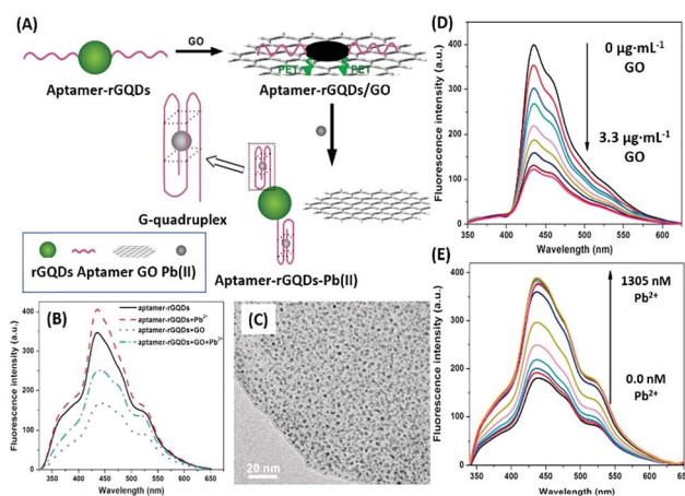
Fig. 6 (A) Schematic illustration of the lead(II) detection strategy of a nanosensor based on photoinduced electron transfer between graphene quantum dots and graphene oxide. (B) The quenching effect of GO nanosheets on aptamer–GQDs, and its restoration in the presence of lead ions. (C) Transmission electron micrograph of the GQD–apta–GO complex. (D) Fluorescence spectra showing quenching of GQDs in the presence of GO in a concentration range of 0–3.3 μg mL −1 . (E) Fluorescence spectra showing restoration of fluorescence upon addition of 0–1305 nM lead ions. Adapted with permission from ref. 93. Copyright (2015) Elsevier.
