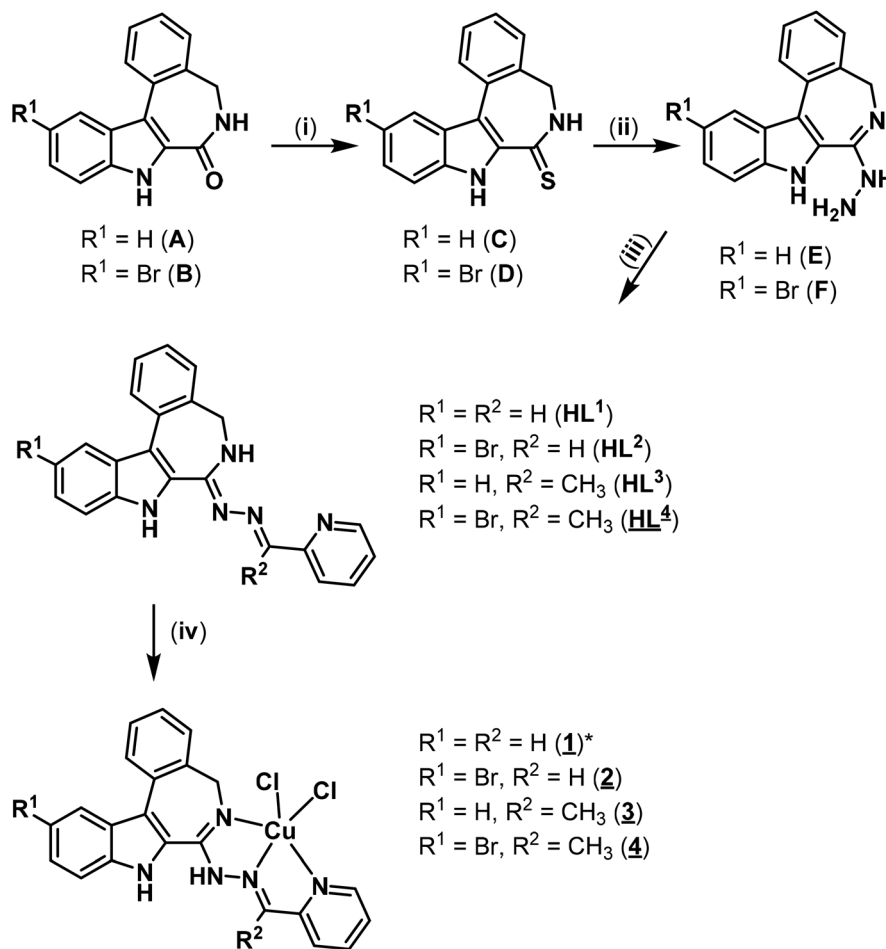
Chart 2 New prolignands and copper(II) complexes synthesised in this work. a Underlined numbers indicate compounds studied by X-ray diffraction. * 1 crystallised from DMF as the trimer [\text{Cu}_3\text{Cl}_4(\text{HL}^1)_3]\text{Cl}_2 ( 1 trim ). a Reagents and conditions: (i) C: phosphorus pentasulfide/aluminium oxide, acetonitrile, 85 °C, overnight; D: phosphorus pentasulfide/aluminium oxide, tetrahydrofuran, 75 °C, overnight; (ii) hydrazine monohydrate, reflux, overnight; (iii) HL 1 , HL 2 : 2-formypyridine, ethanol, 85 °C, overnight; HL 3 , HL 4 : 2-acetylpyridine, ethanol, 85 °C, overnight; (iv) \text{CuCl}_2 \cdot 2\text{H}_2\text{O} , isopropanol, reflux, 15 min.
