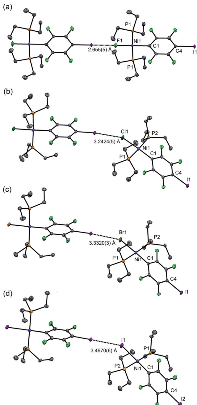
Fig. 1 Molecular structures of 1pX (a) X = F , (b) X = Cl , (c) X = Br , (d) X = I , showing intermolecular halogen bonds. Displacement ellipsoids at 50% probability level. Hydrogen atoms not shown. Three-molecule chains are illustrated in the ESI.†
