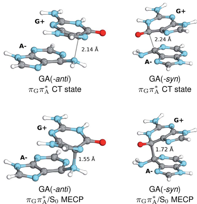
Fig. 5 Geometries of the different G^+A^- S_1 minima located for both GA(-syn) and -anti conformers (top), and the corresponding S_1/S_0 MECPs (bottom). The optimizations were performed using QM bases /MM setup, but only the G and A bases are shown for clarity.
