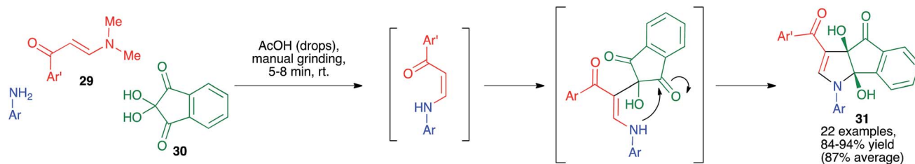
Scheme 20 Three component mechanochemical synthesis of dihydroindeno[1,2-b]pyrrole derivatives.
