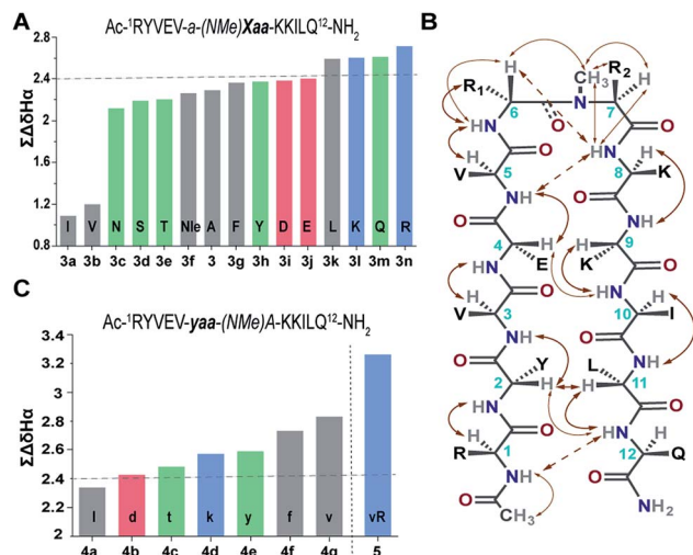
Fig. 4 (A) \Sigma CSD of the primary library with L-amino acid substitutions (Xaa) at the i+2 site. (B) The characteristic NOEs, where the thick arrows denote strong (1.8–2.1 Å), the thin arrows denote medium (2.2–2.5 Å) and the broken arrows denote weak ( >2.6 Å) NOEs. (C) \Sigma CSD of the secondary library with i+1 substitutions (yaa) along with 5 derived from the combination of 4g and 3n. All the NMR measurements were done in acetate buffer (pH 3.8) at 25 °C.
