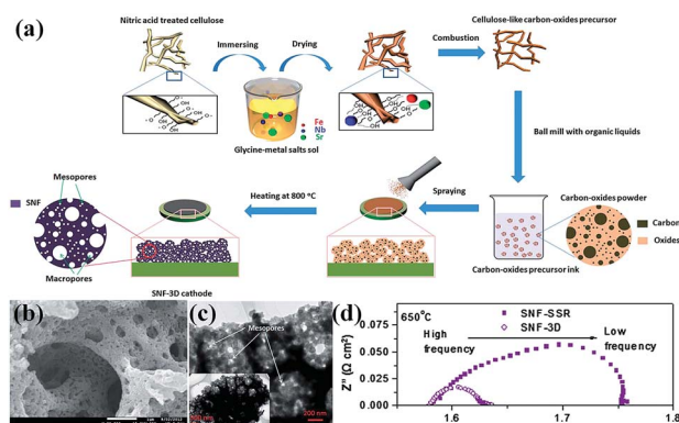
Fig. 5 (a) Procedure for the preparation, (b) SEM and (c) TEM images of a 3D aperiodic hierarchical porous SNF cathode calcined at 800 °C for 2 h in air, and (d) electrochemical impedance spectroscopy of SNF-3D and SNF-SSR (SSR: solid state reaction) at 650 °C. Reproduced with permission from ref. 104. Copyright© 2012, Royal Society of Chemistry.
