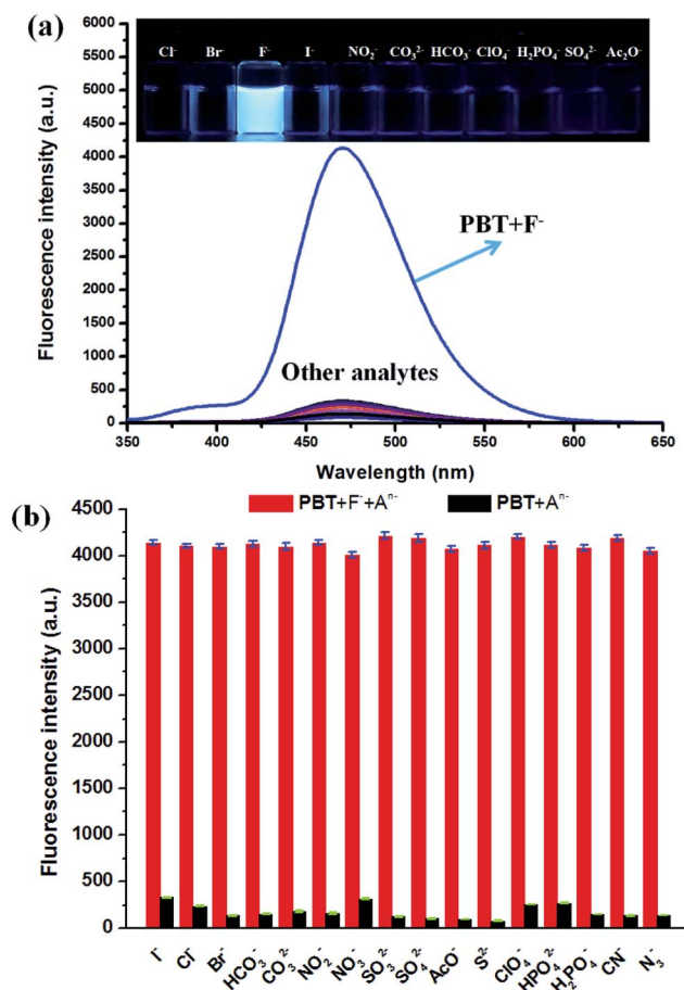
Fig. 6 (a) Fluorescence spectra of PBT in the presence of various anions. [PBT] = 10 \mu M , [ A_n^- ] = 20 \mu M , in a mixture of THF and Tris buffer solution (pH 8.0), (1 : 9, v/v), \lambda_{ex} = 335 nm, \lambda_{em} = 470 nm. Inset: direct observation of fluorescence emission difference of the probe PBT (10 \mu M ) under UV irradiation (365 nm) in the presence of different anions. Left to right: Cl^- , Br^- , I^- , F^- , NO_2^- , CO_3^{2-} , HCO_3^- , ClO_4^- , H_2PO_4^- , SO_4^{2-} and AcO^- . (b) The selectivity of PBT in the presence of various anions.
