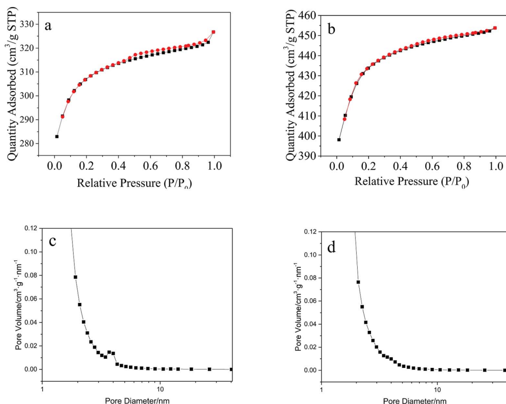
Fig. 5 Nitrogen sorption isotherms: Cu(BTC)-rGO (a), Cu(BTC) (b); pore size distribution: Cu(BTC)-rGO (c), Cu(BTC) (d).
