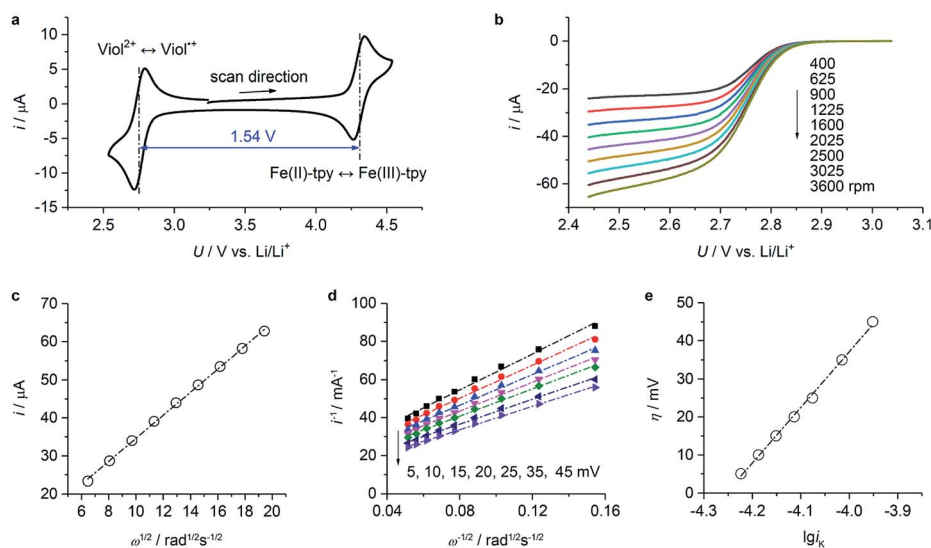
Fig. 3 CV and RDE studies for (\text{CH}_2)_5\text{CH}_3 -substituted \text{Viol}^{2+} . (a) CV profile of (\text{CH}_2)_5\text{CH}_3 -substituted \text{Viol}^{2+} and \text{Fe(II)-tpy} mixed electrolyte in EC/DMC containing 0.25 M \text{LiTFSI} at a scan rate of 10 \text{ mV s}^{-1} . (b) RDE profiles of (\text{CH}_2)_5\text{CH}_3 -substituted \text{Viol}^{2+} in EC/DMC. The electrolyte was composed of 2 mM (\text{CH}_2)_5\text{CH}_3 -substituted \text{Viol}^{2+} , 0.25 M \text{LiTFSI} in EC/DMC. The scan rate was 10 \text{ mV s}^{-1} . (c) Limiting current ( i_{\text{lim}} ) vs. square root of rotation speed ( \omega^{1/2} ) derived from (b). (d) \eta -Dependent current as a function of \omega^{-1/2} derived from (a). (e) \eta as a function of \lg i_K upon the first reduction of (\text{CH}_2)_5\text{CH}_3 -substituted \text{Viol}^{2+} . The x-intercept provides the log of i_0 .
