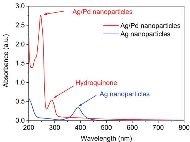
Fig. 3 UV-vis spectra of Ag nanoparticles formed after Reactor 2 and Ag–Pd bimetallic nanoparticles formed in Reactor 3 using \text{K}_2\text{PdCl}_4 as precursor.
