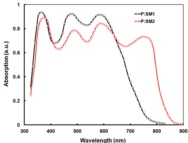
Fig. 4 Normalized absorption spectra of P:SM1 and P:SM2 in thin films cast from chloroform.
