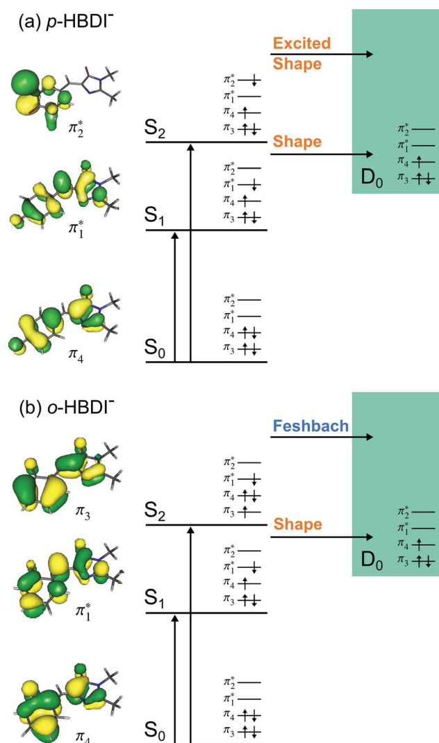
Fig. 6 Energy level diagram of (a) p -HB \text{BDI}^- and (b) o -HB \text{BDI}^- in which possible excitations and subsequent detachment processes are indicated (note that it is only the vibrationally excited states of S_1 lying in the D_0 continuum that have shape resonance character). S_1 and S_2 refer to the first two excited states selected in Table 2. The HOMO is \pi_4 and the LUMO is \pi_1^* . Alongside are the Hartree–Fock molecular orbitals that are involved in the excitations. For op -DH \text{BDI}^- , a similar scheme applies as for p -HB \text{BDI}^- except the excited state resonance is S_3 (Table 2).
