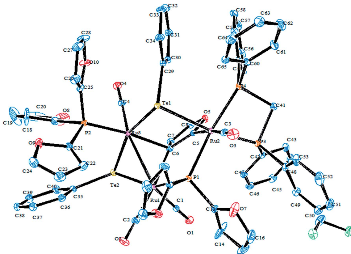
Fig. 6 Crystal structure of [\text{Ru}_3(\mu_3\text{-}\eta^2\text{-C}_4\text{H}_3\text{O})((\mu\text{-PC}_4\text{H}_3\text{O})_2)(\text{CO})_5(\mu\text{-TePh})_2(\mu\text{-dppm})] (redrawn from ref. 103).
