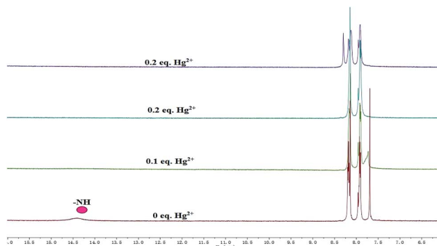
Fig. 7 Partial ^1\text{H} NMR spectra of Z-3 in DMSO- \text{d}_6 with different concentrations of \text{Hg}^{2+} .
