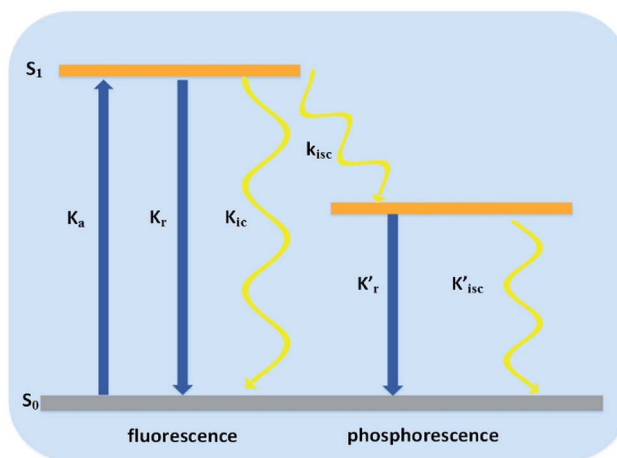
Fig. 12 Elementary photophysical processes of molecular luminescence. 68
