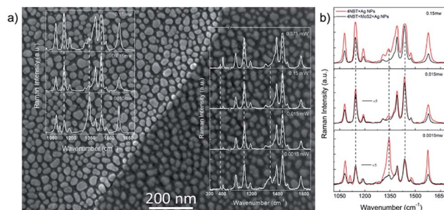
Fig. 27 (a) The substrate for the contrast experiments and the SERS spectra are shown. There are only Ag NPs on the left, while the NPs are covered by \text{MoS}_2 on the right. (b) The surface catalytic reactions for the 25 nm NPs with \text{MoS}_2 (black line) and without \text{MoS}_2 (red line). 105
