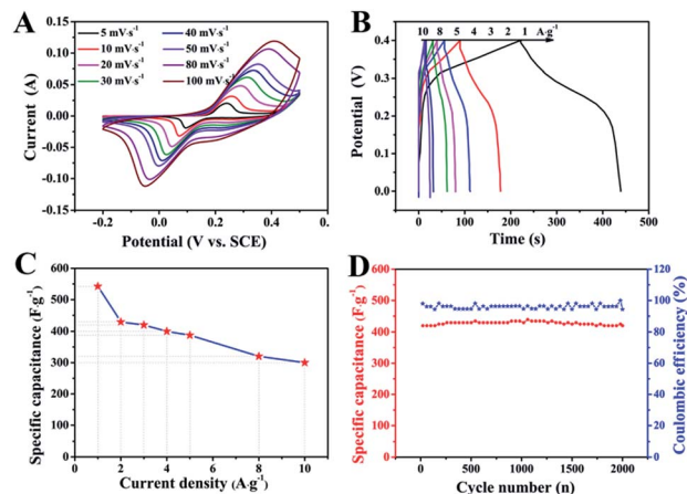
Fig. 5 The electrochemical test results of the \text{ZnCo}_2\text{O}_4 microsphere electrode. (A) The CV curves at various scan rates. (B) The GCD curves at various current densities. (C) The capacitance as a function of current density. (D) The cycling performance and Coulomb efficiency at 2 \text{ A g}^{-1} .
