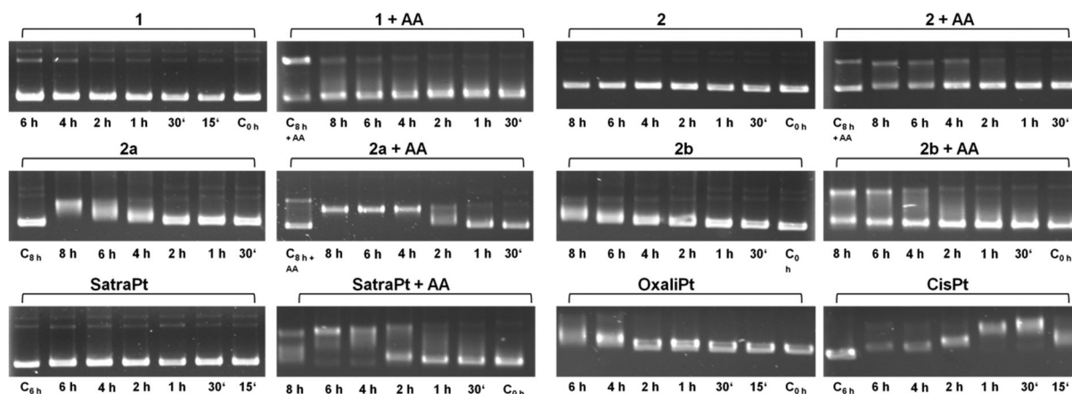
Fig. 2 Electropherograms of dsDNA plasmid pUC19 incubated with 50 \mu M of platinum(IV) compounds 1, 2, 2a, 2b or satraplatin (in the absence or presence of 500 \mu M ascorbic acid, AA), oxaliplatin or cisplatin for different incubation times at 37 ^{\circ} C in TE buffer (pH = 7.8).
