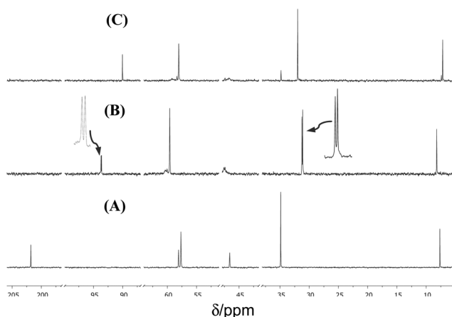
Fig. 2 Partial ^{13}\text{C} NMR (100.6 MHz; 25 °C) spectra of (1a) (15 mM) in: (A) \text{dms}-d_6 ; (B) \text{CD}_3\text{OD} ; expansions are shown next to two peaks; and (C) \text{D}_2\text{O} . The solvent peaks were removed for clarity.
