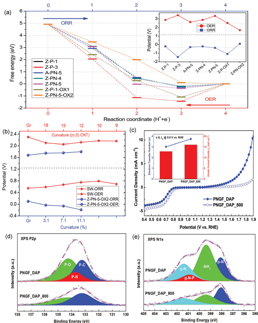
Fig. 3 (a) Free energy variations of ORR/OER elementary steps for different P containing structures. (b) ORR/OER limiting potentials for Z-PN-5-OX2 and Stone–Wales defect structures. (c) Bifunctional ORR/OER activities of PNGF_DAP and PNGF_DAP_800 (inset: the electron transfer number and kinetic current density for ORR at 0.6 V vs. RHE). XPS (d) P2p and (e) N1s spectra for PNGF_DAP and PNGF_DAP_800.
