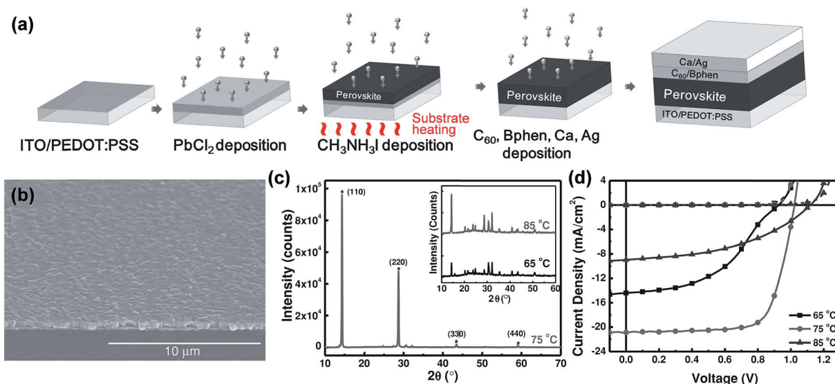
Fig. 8 (a) Schematic illustration for the fabrication of perovskite solar cell employing sequential layer-by-layer vacuum deposition. (b) Large area SEM image of the CH 3 NH 3 PbI 3-x Cl x thin film fabricated with the substrate temperature held at 75 °C during CH 3 NH 3 sublimation. (c and d) XRD and J–V characteristics of perovskite layers and solar cells with varying substrate temperatures (65 °C, 75 °C, 85 °C) during CH 3 NH 3 sublimation. Reproduced with permission from ref. 88.
