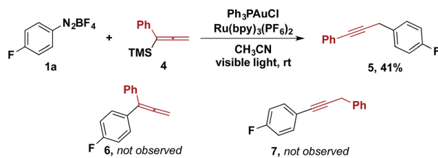
Scheme 2 Reaction with allenyltrimethylsilanes.
