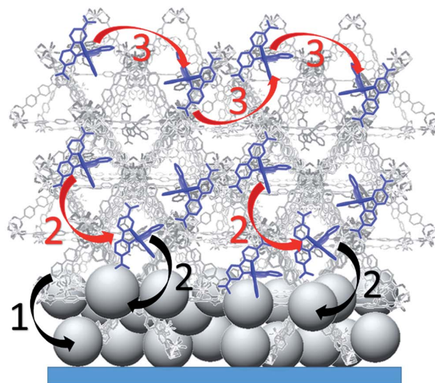
Fig. 4 (Left) Front-side solar cell sandwich arrangement used for the photovoltaic cells prepared here. (Right) General scheme depicting the potential processes contributing to the observed photocurrent for the RuDCBPY-MOF modified \text{TiO}_2 films. The black arrows indicate charge separation steps whereas the red arrows are indicative of energy transfer/hopping between RuDCBPY centers within the MOF. (1) Charge separation between the BPDC or DCBPY MOF ligands and \text{TiO}_2 . (2) Charge separation between RuDCBPY centers at or within the energy hopping diffusion length from the MOF/ \text{TiO}_2 interface and the \text{TiO}_2 . (3) Non-directional energy transfer/hopping between RuDCBPY centers within the MOF.
