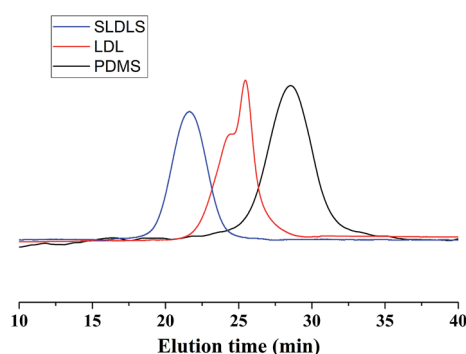
Fig. 3 GPC curves of PDMS, PCL- b -PDMS- b -PCL and PS- b -PCL- b -PDMS- b -PCL- b -PS block copolymers.
