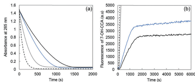
Fig. 5 (a) Ascorbate consumption by Cu-Aβ 28 (black curve), Cu-Aβox (blue curve), Cu-Aβ 7 (grey curve) and free Cu (dashed curve) measured using UV spectrophotometry ( λ = 265 nm) as a function of the reaction time; phosphate buffered solution (50 mM, pH 7.4), Cu(II) 10 μM, peptide 12 μM and ascorbate 100 μM. (b) Fluorescence as a function of the time of 7-OH-CCA resulting from the oxidation of CCA obtained for Cu-Aβ 28 (black curve), Cu-Aβox (blue curve), Cu-Aβ 7 (grey curve) and free Cu (dashed curve); phosphate buffered solution (50 mM, pH 7.4), Cu(II) 50 μM, peptide 60 μM (oxidized or non-oxidized), ascorbate 500 μM and CCA 500 μM.
