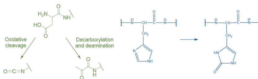
Fig. 2 Amino acid sequence of the A \beta 28 peptide (top) along with the main targeted amino acid residues (in color) and the chemical structure of the oxidation products (bottom). Asp1 oxidation leads to the formation of either an isocyanate or a pyruvate function 21,25 (green) and His13 and His14 oxidation reactions lead to the formation of 2-oxohistidines 21,23,24 (blue).
