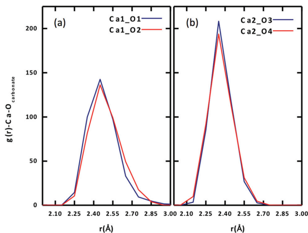
Fig. 3 Radial distribution functions of equatorial carbonate oxygen (O eq ) around each Ca ion of the \text{Ca}_2\text{UO}_2(\text{CO}_3)_3 complex in water (0.53 M): (a) Ca1; (b) Ca2. See Fig. 1 for atom labels.
