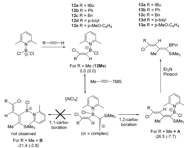
Scheme 4 1-Boradiene formation by haloboration and 1,2-carbaboration. Electronic energies (Gibbs free energies at 293 \text{ K} ) shown in \text{kcal mol}^{-1} for the model system where \text{R} = \text{Me} (all energies relative to 12Me and 1-TMS-1-propyne at infinite distance).
