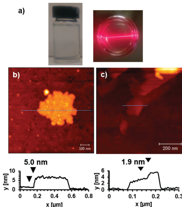
Fig. 2 (a) Images showing a suspension of \text{Cu}(1) nanosheets in DMF with characteristic Tyndal Scattering of laser light. AFM images and height profiles corresponding to blue lines for nanosheets formed by exfoliation of (b) \text{Zn}(1) in DMF (c) \text{Cu}(1) in \text{H}_2\text{O} .
