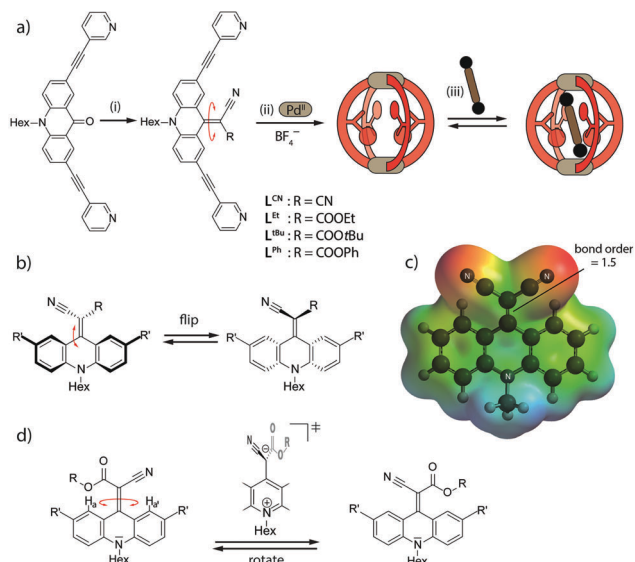
Fig. 1 (a) Ligand synthesis, cage assembly and guest uptake: (i) malonic acid derivative, TiCl_4 , base, CH_2Cl_2 (details see ESI†) (ii) L^R , [Pd(CH_3CN)_4](BF_4)_2 , CD_3CN , (iii) bissulfonate guest ( NBu_4 salt). (b) Flipping of the endohedral attachments, (c) electrostatic potential map of the dicyano ligand L^{CN} highlighting the partial charge separation and C=C double-bond weakening in the push–pull backbone, (d) rotation of the endohedral functionality via a charge-separated transition state.
