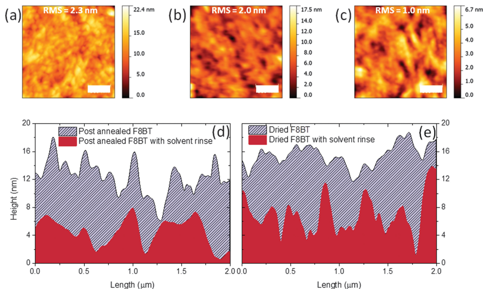
Fig. 2 2 \times 2 \mu\text{m} AFM images of (a) slow cooled F8BT after annealing above T_m , (b) after cyclohexanone spin-rinse (c) following TFB addition (d and e) roughness profiles of annealed and dried at 90^\circ\text{C} F8BT showing the reduction in roughness observed after solvent rinse.
