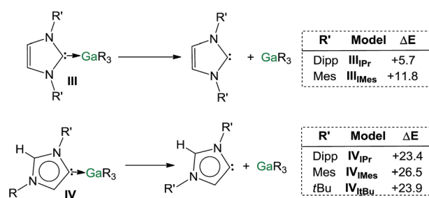
Fig. 7 Estimated dissociation energies ( \text{kcal mol}^{-1} ) of complexes III and IV ( \text{R} = \text{Dipp, Mes, } ^t\text{Bu} ).
