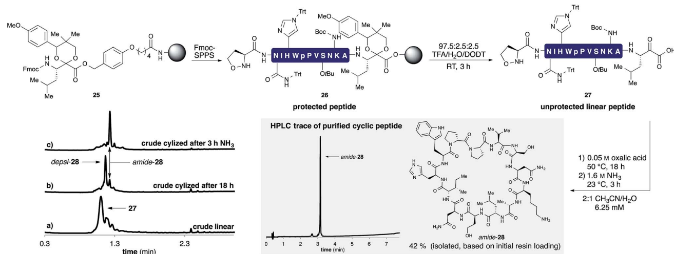
Scheme 5 Synthesis of cyclic peptide amide-28 using the optimized KAH cyclization process. Analytical HPLC traces at 220 nm: (a) crude linear peptide 27 after cleavage from resin. (b) Crude cyclic peptide depsi-28 after 18 h at 50 °C. (c) Crude cyclic peptide amide-28 3 h after the addition of 1.6 M aq \text{NH}_3 . [DODT = 3,6-dioxa-1,8-octanedithiol]. 28
