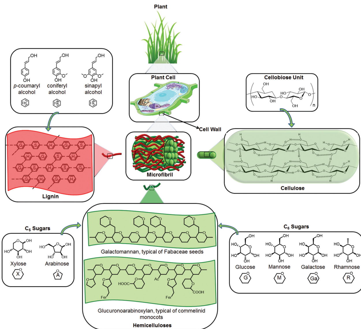
Fig. 1 The main components and structure of lignocellulose. "Gl" represents glucuronic acid and "Fe" represents esterification with ferulic acid, which is characteristic of xylans in commelinid monocots. 28
