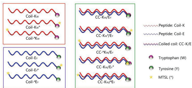
Scheme 1 Schematic illustration of designed peptides and coiled coil motifs. Coil-K peptides are labeled with a tryptophan (W) residue while Coil-E peptides are decorated with a tyrosine (Y) residue. In this paper W and Y are always at the C-terminus of the peptides. A yellow star represents the MTSL- (*) nitroxyl radical spin label, which is added to either the C- or the N-terminus, to investigate the possibility of CC-K/E parallel and antiparallel orientations respectively. See Table 1 for primary sequences of all peptides.
