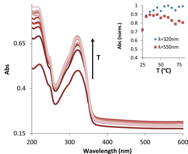
Fig. 2 Absorption spectra of 1 (38 \mu M in water) at different temperatures.
