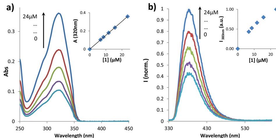
Fig. 1 (a) Absorption spectra at different concentrations of 1 in methanol. Inset: absorbance at 320 nm vs. concentration of 1 ; (b) fluorescence spectra at different concentrations of 1 in methanol. Inset: intensity ( I ) at 383 nm versus concentration of 1 . \lambda_{exc} = 320 nm.
