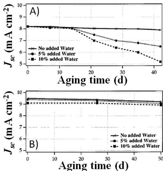
Fig. 17 Long-term stability ( P_{\text{in}} = 0.015 \text{ mW cm}^{-2} ) of DSSCs assembled with RTIL-based electrolytes ( \text{I}_2 10 mM in HMIL) encompassing different \text{H}_2\text{O} contents. Dyes: (A) N3; (B) [\text{Ru}(\text{H}_2\text{dcbpy})(\text{mhdcbpy})(\text{NCS})_2] . Adapted and reprinted from ref. 231.
