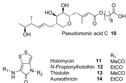
Fig. 1 Thiomarinol, pseudomonic acid and acyl pyrrothine antibiotics.
