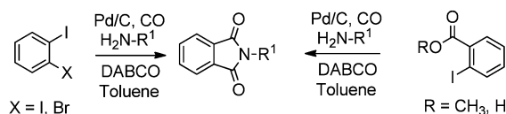
Scheme 28 Reagents and conditions: o-dihaloaryl/o-halobenzoate/o-halobenzoic acid (0.5 mmol), amine (0.7 mmol), 10% Pd/C (2.5 mol%), DABCO (1.5 mmol), toluene (7 mL), CO (90 psi), temp. 120 °C, time 2 h.
